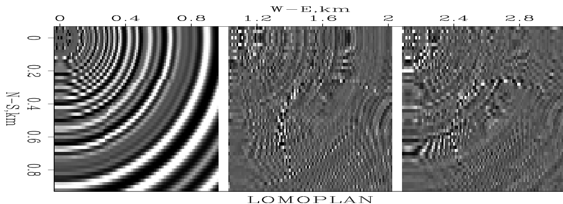
Figure 1.9: Left is a horizontal slice through the 3-D qdome model. Center is the in-line component of the LOMOPLAN. Right is the cross-line component of the LOMOPLAN. Press button for volume view. [CR]
