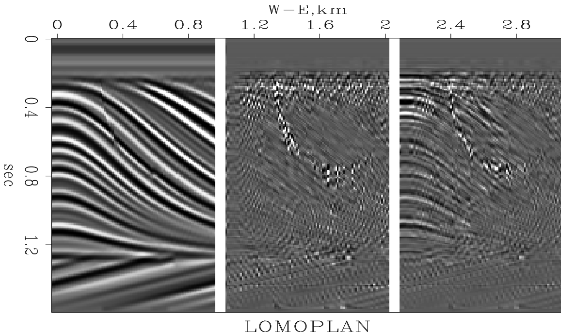
Figure 1.8: Left is a vertical slice through the 3-D “qdome” model. Center is the in-line component of the LOMOPLAN. Right is the cross-line component of the LOMOPLAN. lmn-qdomesico90 [CR]
