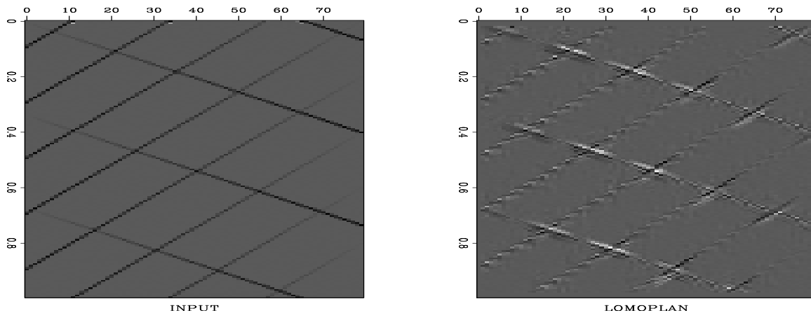
Figure 1.5: Conflicting dips before and after application of a local monoplane annihilator. Press button for movie. The movie sequence is: 1: data, 2: data after LOMOPLAN, 3: like previous but windows not overlapping, 4: predicted data lmn-conflict90 [ER]
