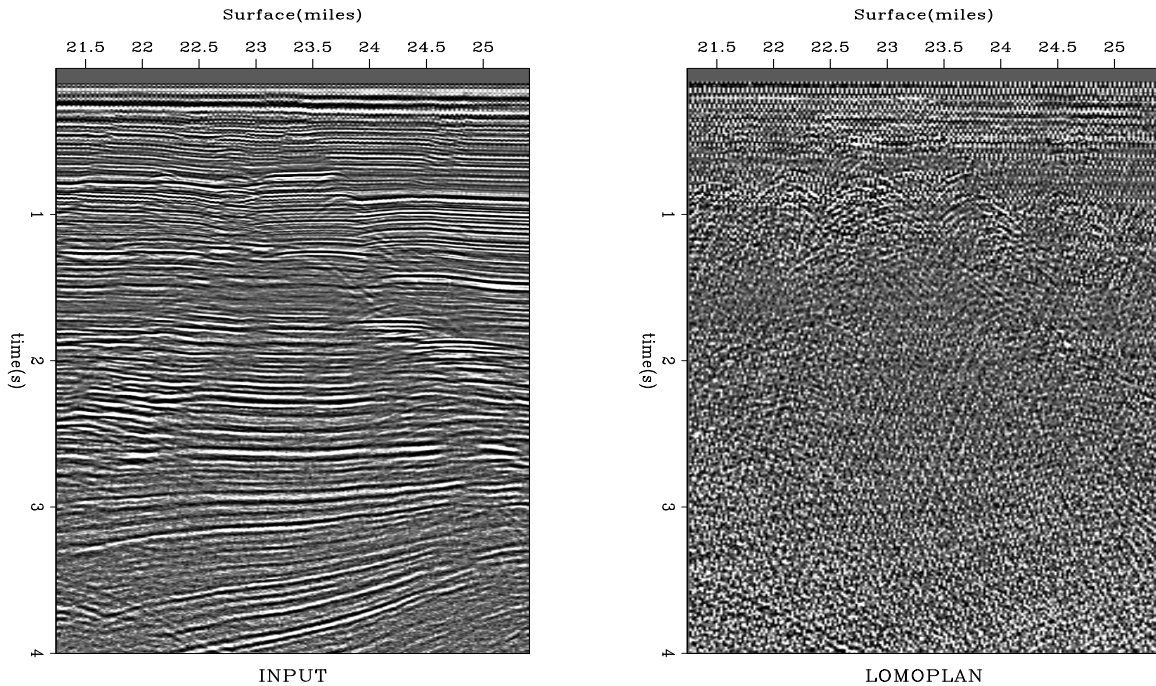
Figure 1.6: Data section from the Gulf of Mexico (left) and after LOMOPLAN (right) Press button for movie. lmn-dgulf90 [ER]
